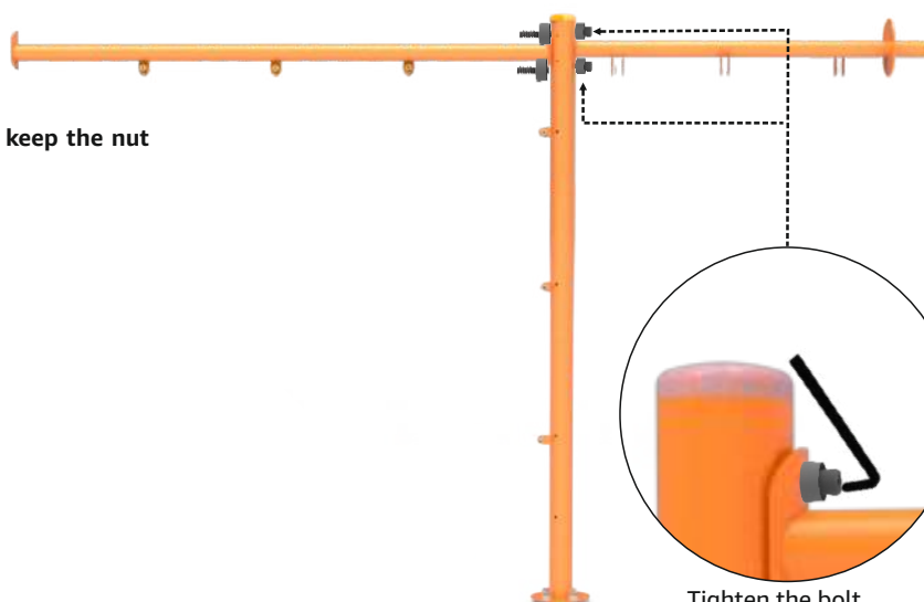
Tighten the bolt with allen key
