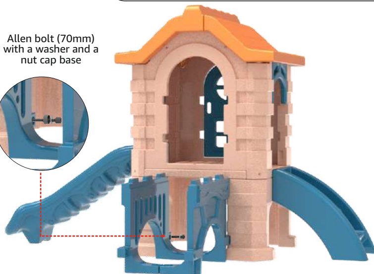
Subassembly (Step 7)
